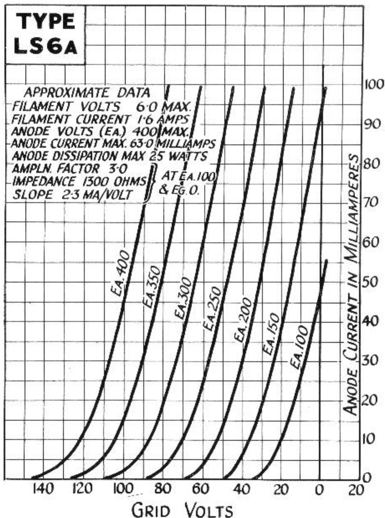
Characteristic Curve of Average LS 6a Valve.
